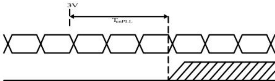
LVDS timing(2)
