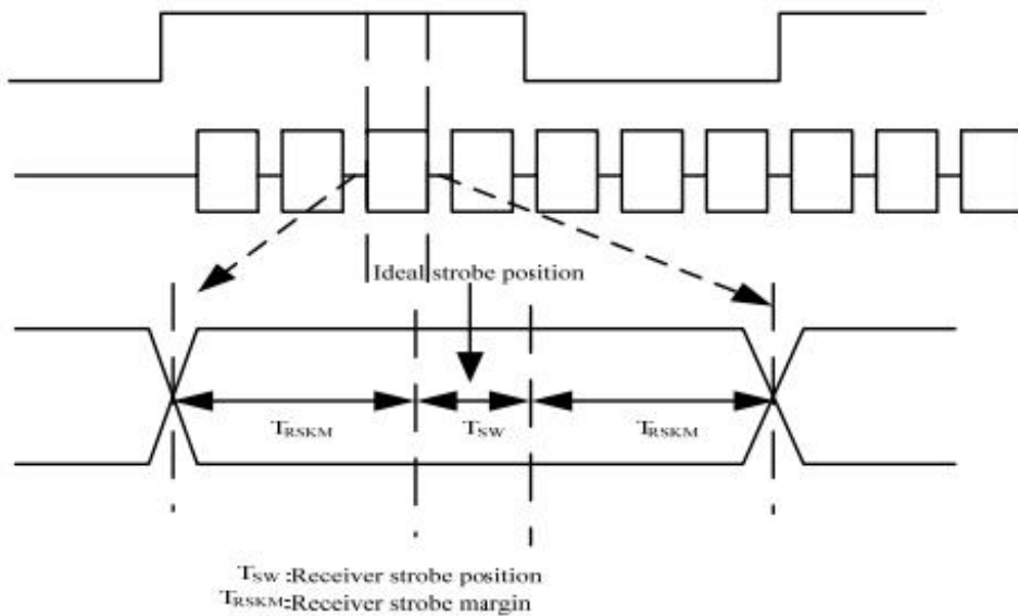
LVDS timing(2)
