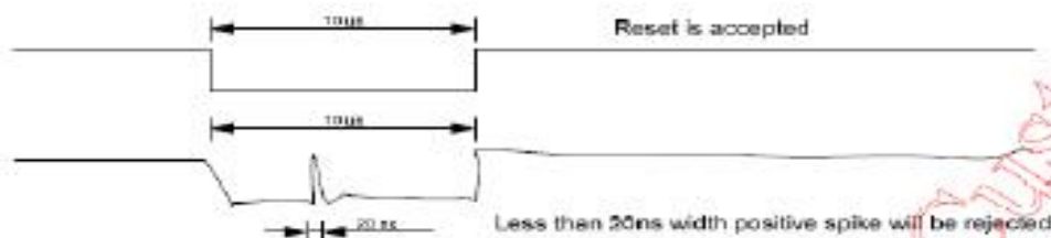
Positive Noise Pulse during Reset Low
