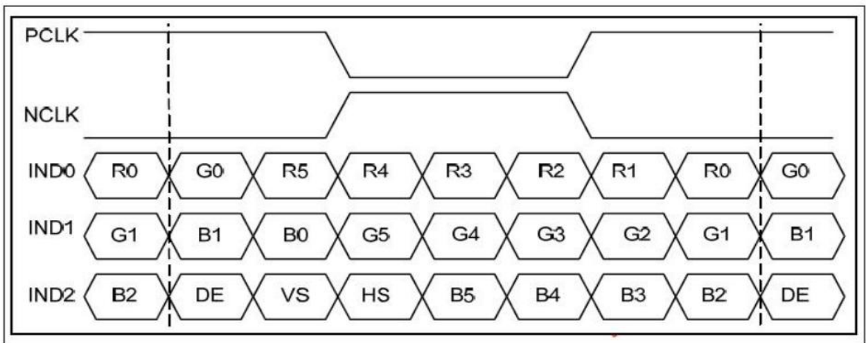
6-bit LVDS Input timing chart
