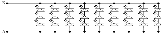
Backlight Circuit diagram
