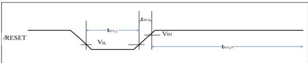
Reset timing
