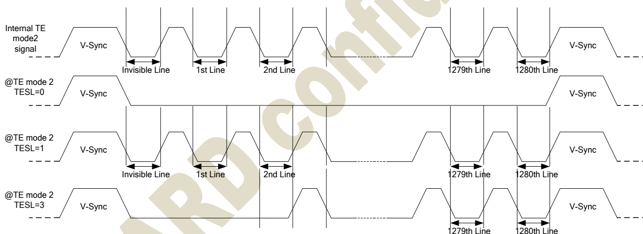
Figure 9.4: TE Line Output for TELINE setting
