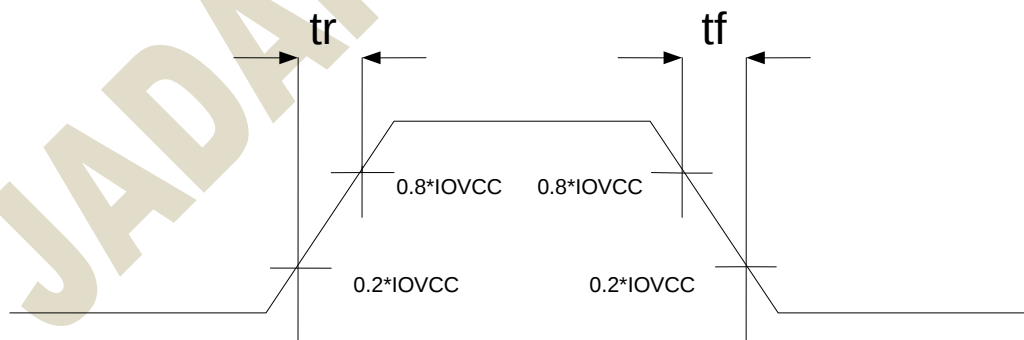
Figure 9.7: Tearing Effect Line definition of t_f , t_r
