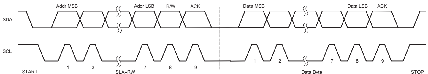
Figure B-6. Byte Transmission
