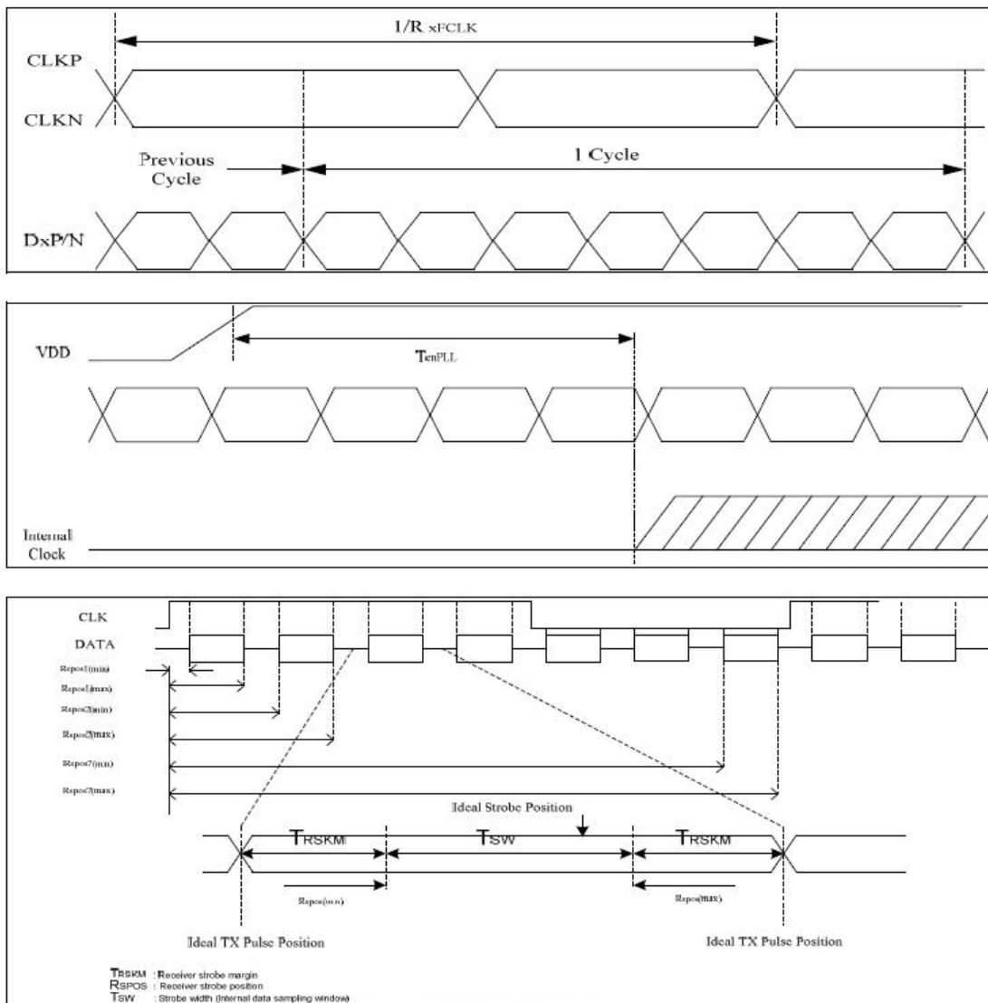
Figure 13.3: LVDS figure
