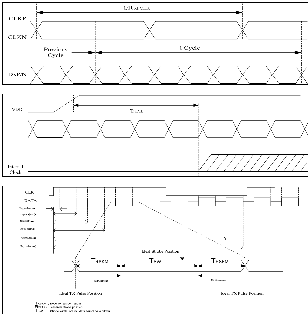
Figure 13.3: LVDS figure
